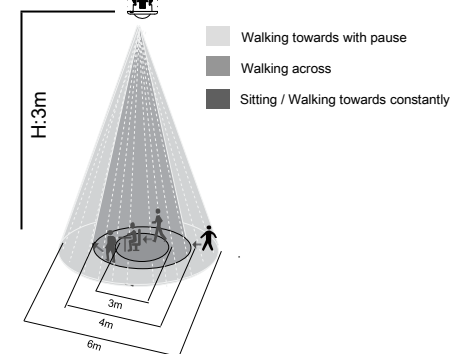
Detection Range (At 25°C)
