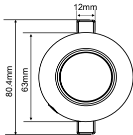
Figure 2. Dimensions-Front View
