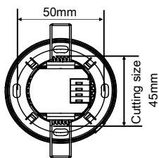
Figure 4. Dimensions-Back View
