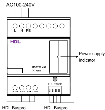
Figure 4. Wiring
