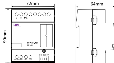
Figure 2. Dimensions - Front View
