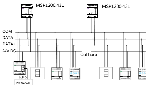
Figure 5. Wiring
